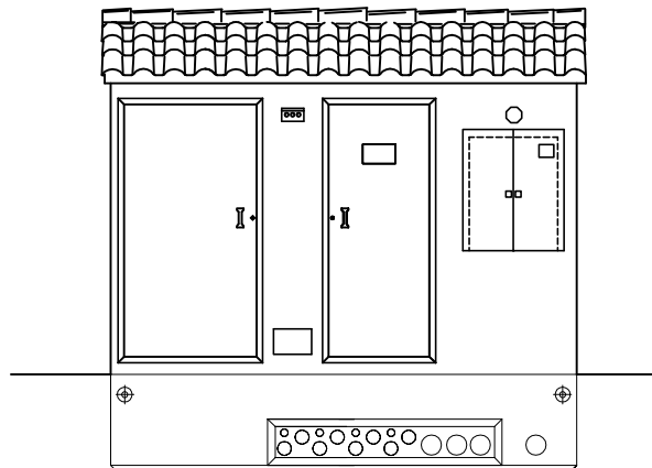
FACADE AVANT.
