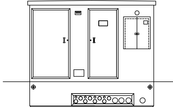
FAÇADE AVANT.
