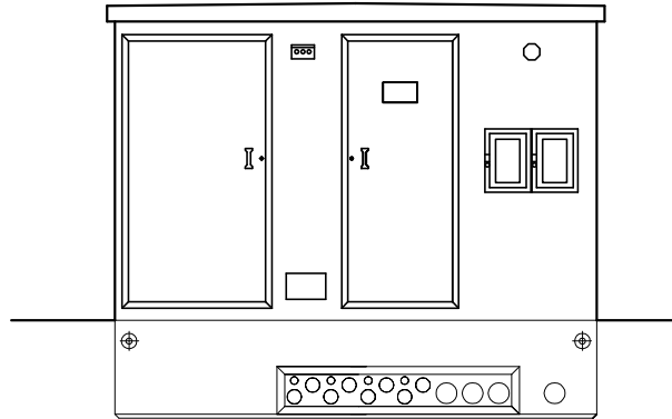
FAÇADE AVANT.
