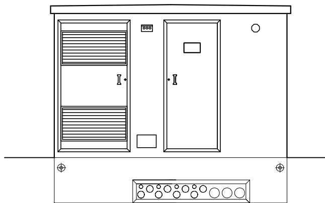
FAÇADE AVANT.
